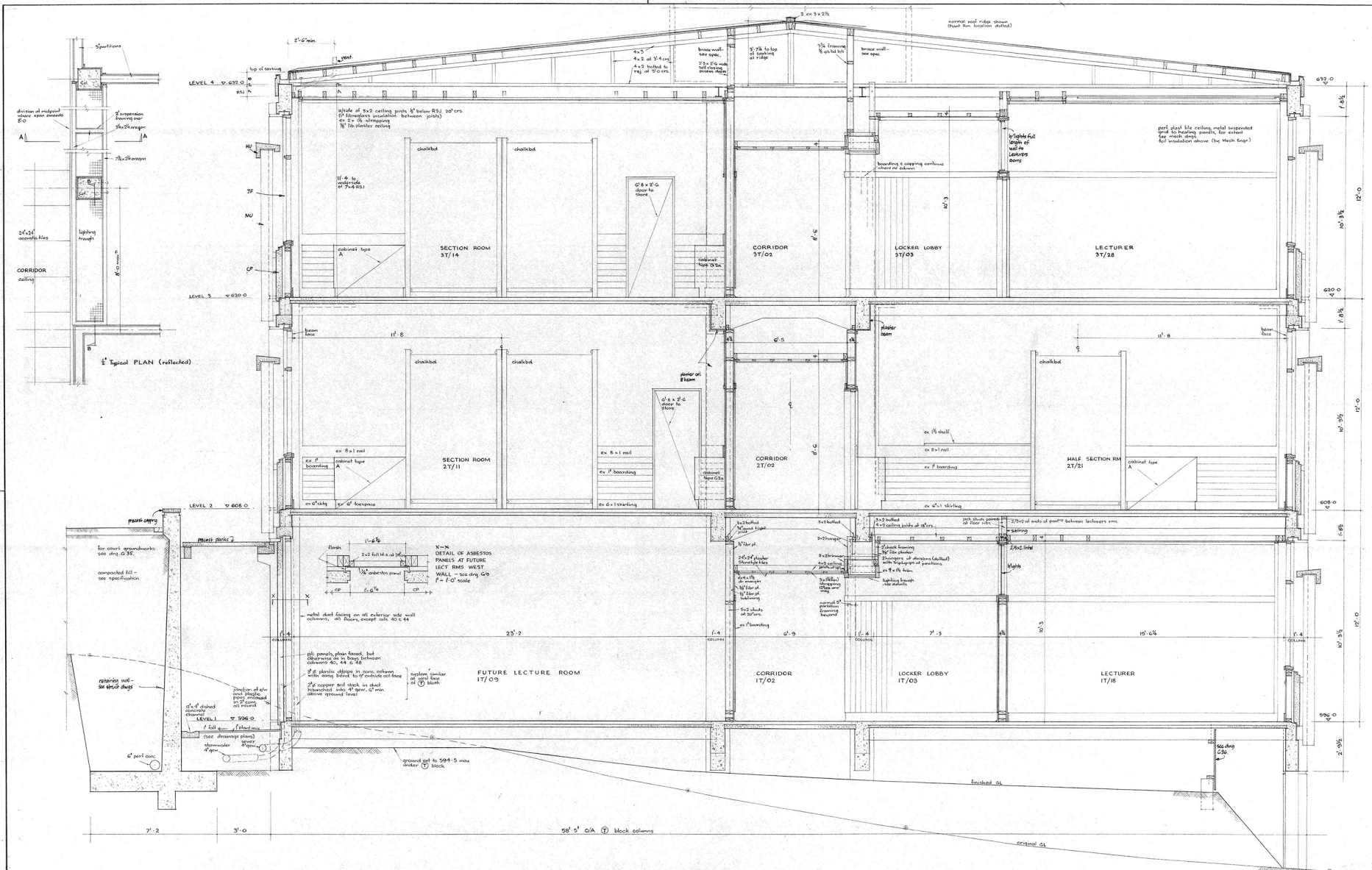
T BLOCK : TYPICAL SECTION LOOKING SOUTH 1/4" = 1'-0" scale (for location see 1/8" scale plans, central core)
